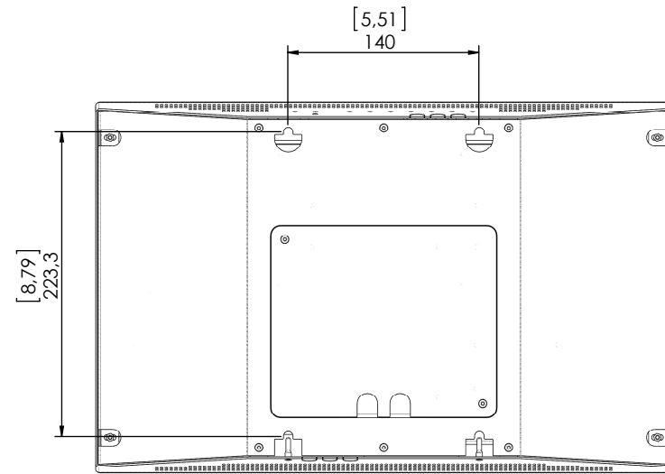
WALL SCREWS PATTERN (140 x 223,3)
