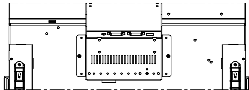
DETAIL C - CONNECTIONS ESCALA 1 : 5
