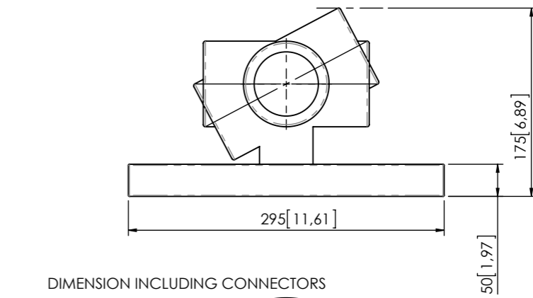
MAXIMUM CAMERA DIMENSIONS
